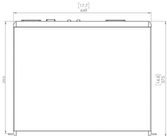
Figure 2 – CCU100 dimensions
